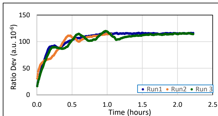
Figure 2. Measurement of a standard 0.001 \Omega shunt vs. a 1 \Omega standard resistor, with a measurement current of 100 A and a 2 hour wait between runs.
