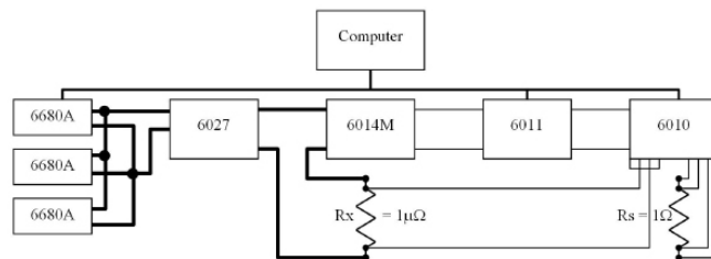
6014M used as range extender with the 6010
